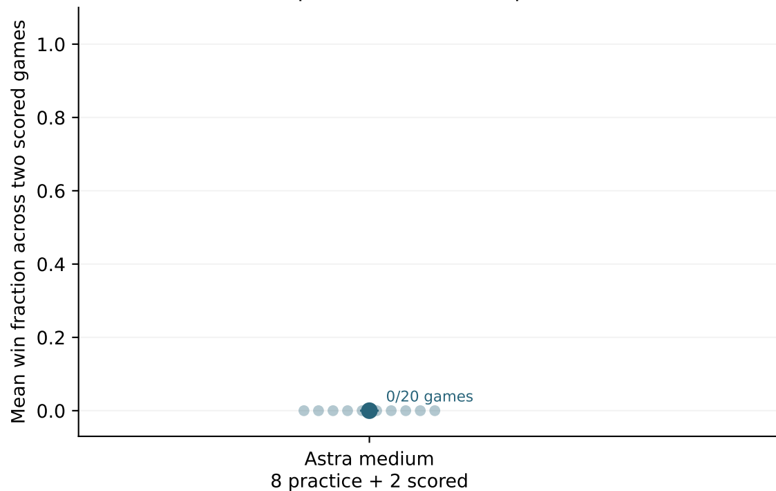
95% bootstrap interval over independent sessions
