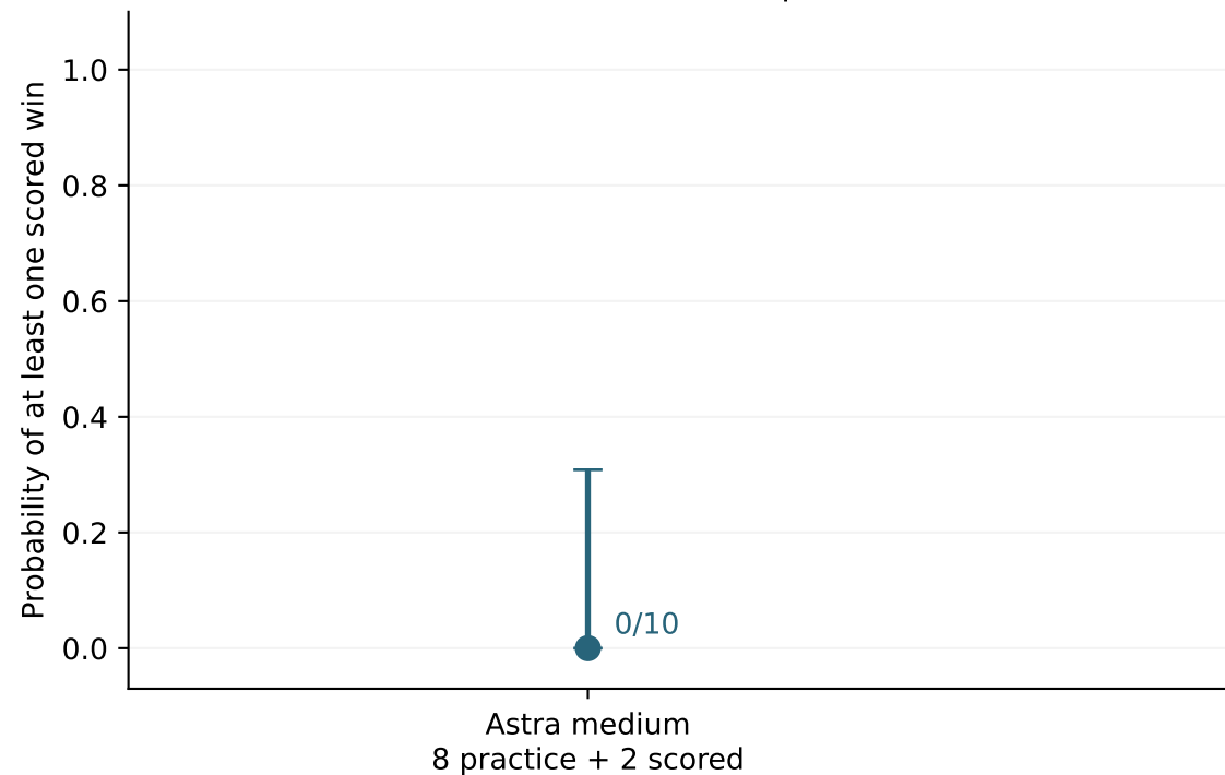
Exact 95% interval over independent sessions
